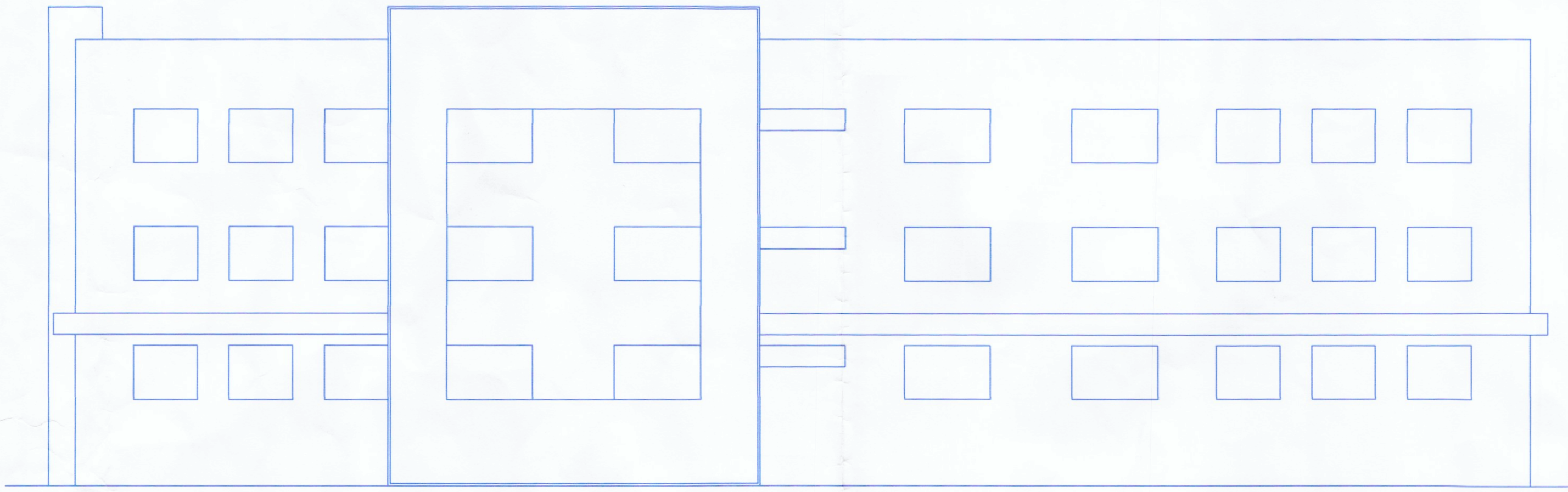
WEST-SIDE ELEVATION 1:100
