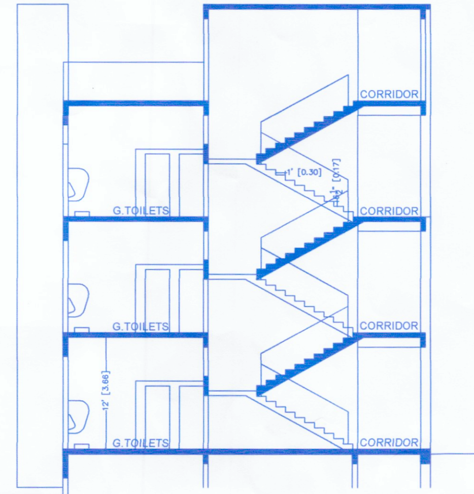
SECTION [PART] AT 'AA' 1:100
